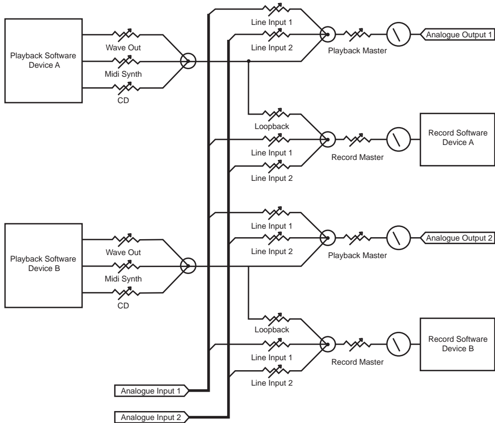
Fig 1-4: Auricon 4.4 Topology
