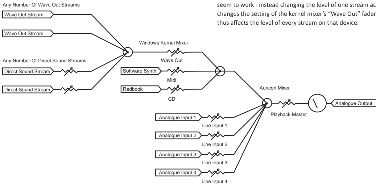
Fig 1-5: Output Mixing
