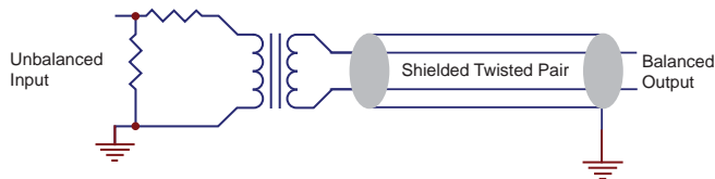
Fig 1-1: Connecting the Auricon 4.4 to Unbalanced Inputs
