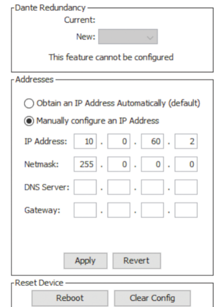
Fig 9: Dante Controller - Network Config in Device View
