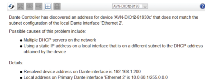
Fig 7: Error details
